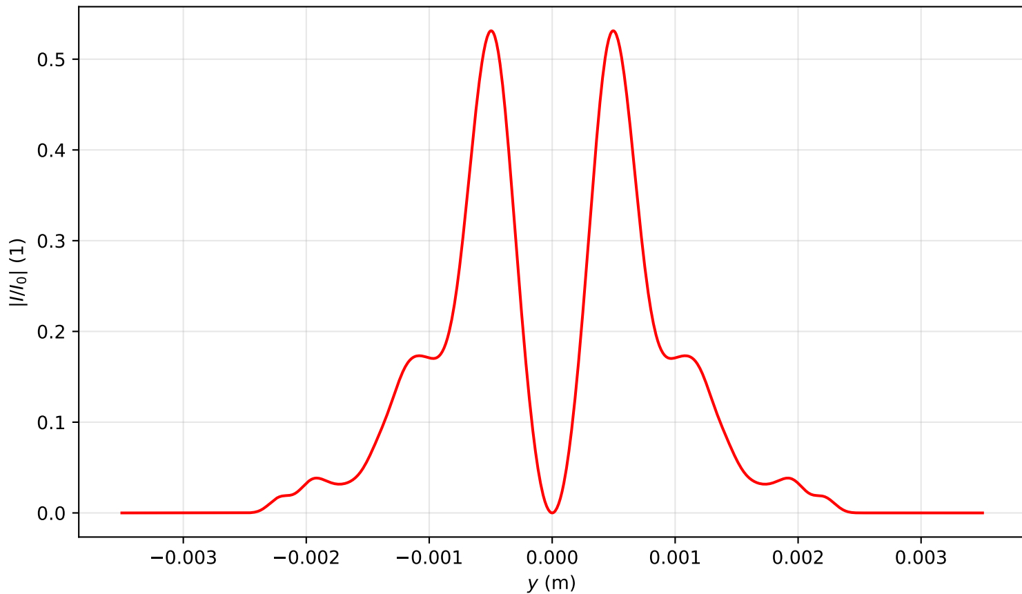
Intensity profile I(x=0, y, z=2.627)/I_0 , P_{in}=5.0P_{cr} , artificial time
